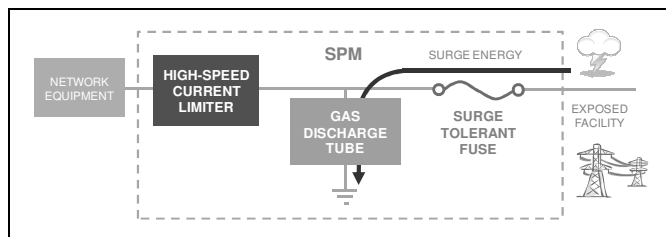
Figure 2. SPM block diagram
